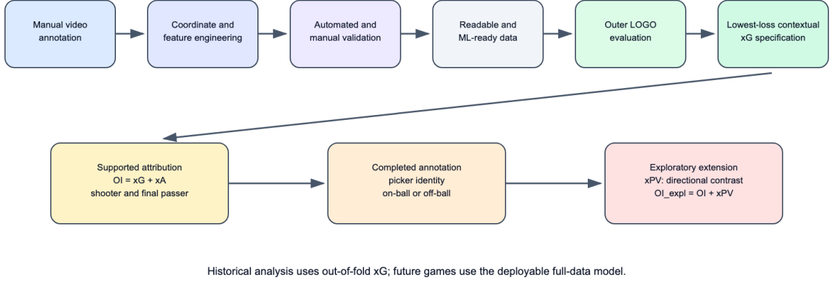
Figure 2: Data-preparation and modeling workflow. Manually annotated events undergo feature engineering, validation, and encoding before model development and downstream offensive analysis.
